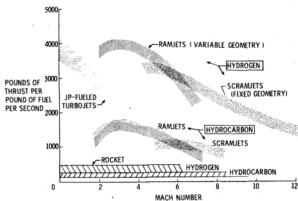
Figure 12. Propulsion Options
