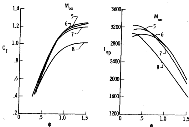
Figure 13. Scramjet Installed Performance
