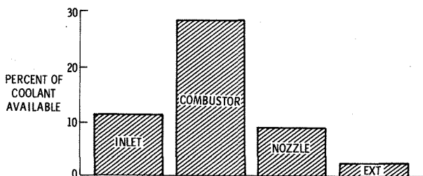
Figure 15. Engine Heat Load; M_\infty = 6 , q_\infty = 500 psf
