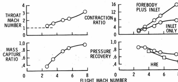
Figure 4. Inlet Aerodynamics
