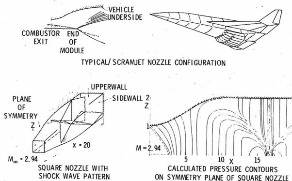
Figure 6. Integrated Scramjet Nozzle
