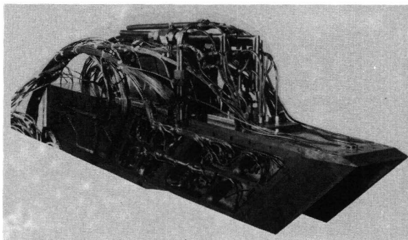
Figure 7. Instrumented Subscale Scramjet Module
