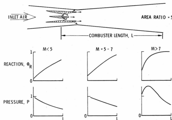
Figure 5. Combustor Operation
