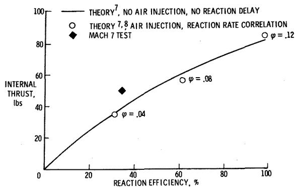
Figure 11. Predicted Internal Thrust
