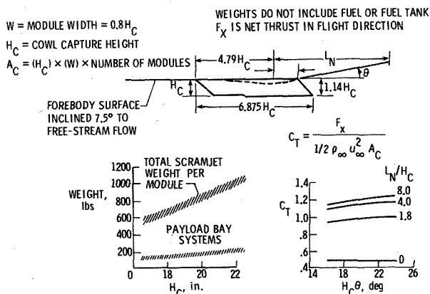
Figure 14. Scramjet Weight and Nozzle Geometry
