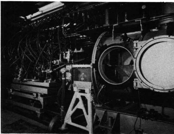
Figure 9. Mach 7 Scramjet Test Facility
