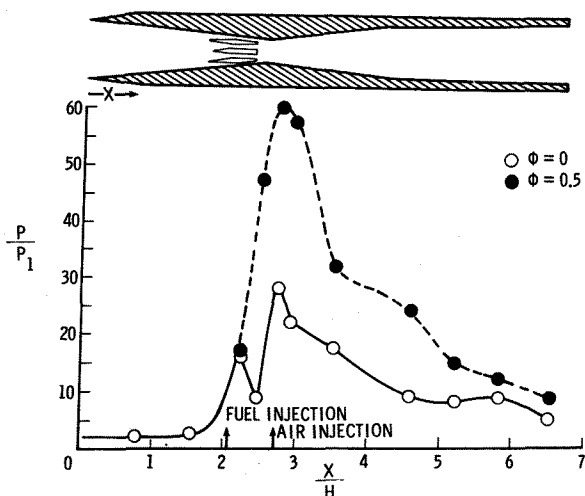
Figure 10. Internal Sidewall Pressure Distribution (Mach 7 Flight Simulation)
